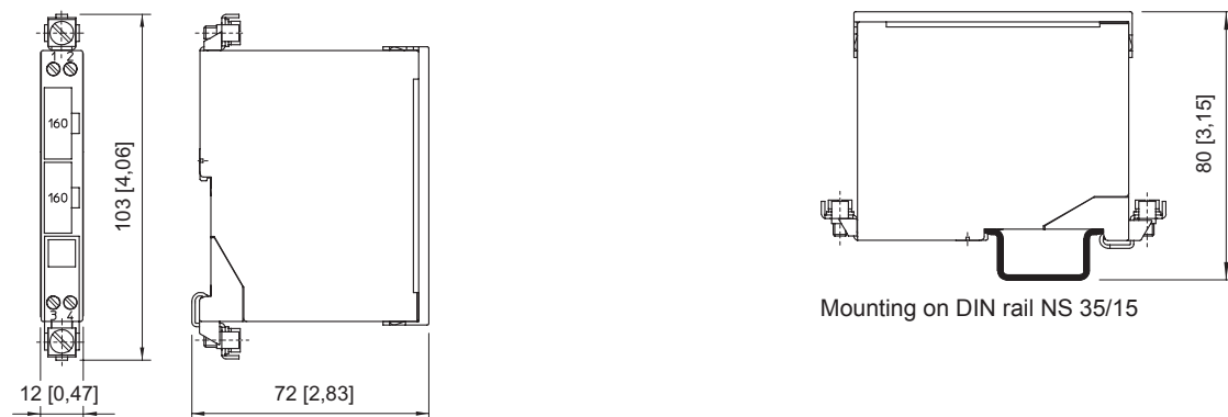
Two-channel safety barriers, potential: - / -
